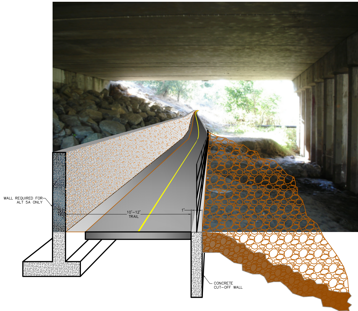
TYPICAL TRAIL SECTIONS UNDER SUNRISE BRIDGE SEGMENT 5 – SUNRISE ALTERNATIVES 5A, 5B AND 5C
