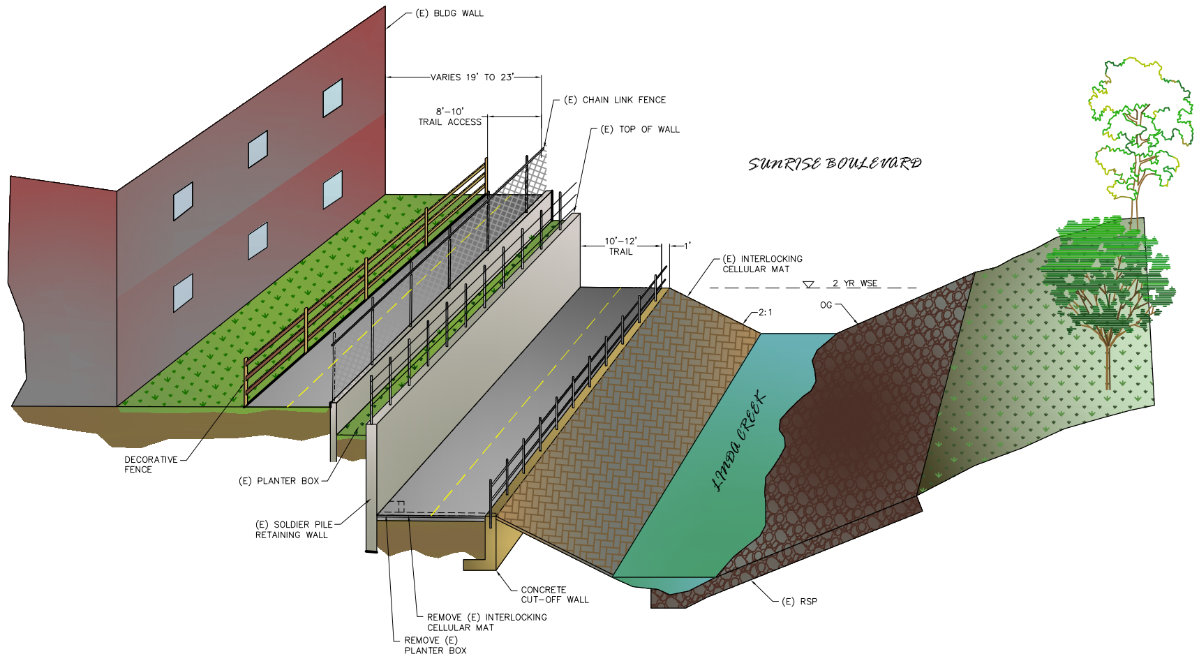
TYPICAL TRAIL SECTIONS ALONG FLOODWALLS SEGMENT 5 – SUNRISE ALTERNATIVES 5B AND 5C
