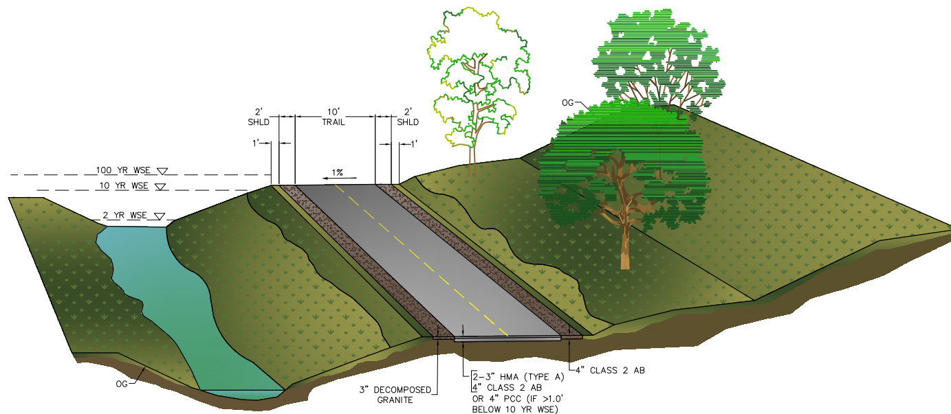
TYPICAL TRAIL SECTION SEGMENTS 1 AND 5 ADJACENT TO CREEK IN FLOODPLAIN
